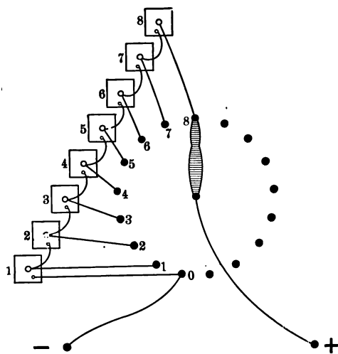
Plan of current collector.
